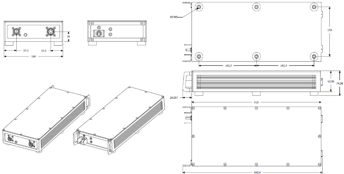
Figure 1: Mechanical Dimensions
